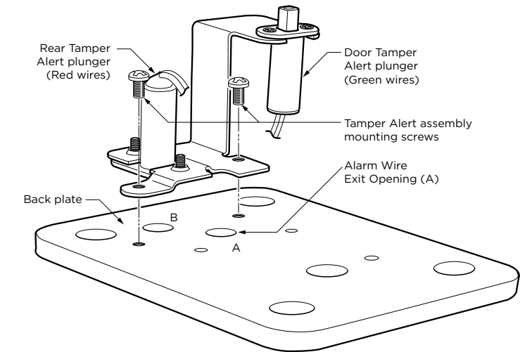
Tamper Alert Assembly
