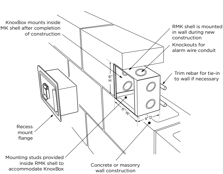
Recess Mounting Using Recess Mounting Kit
