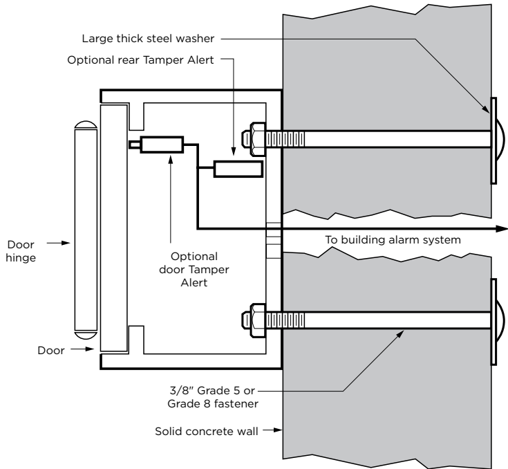
Surface Mounted Models
