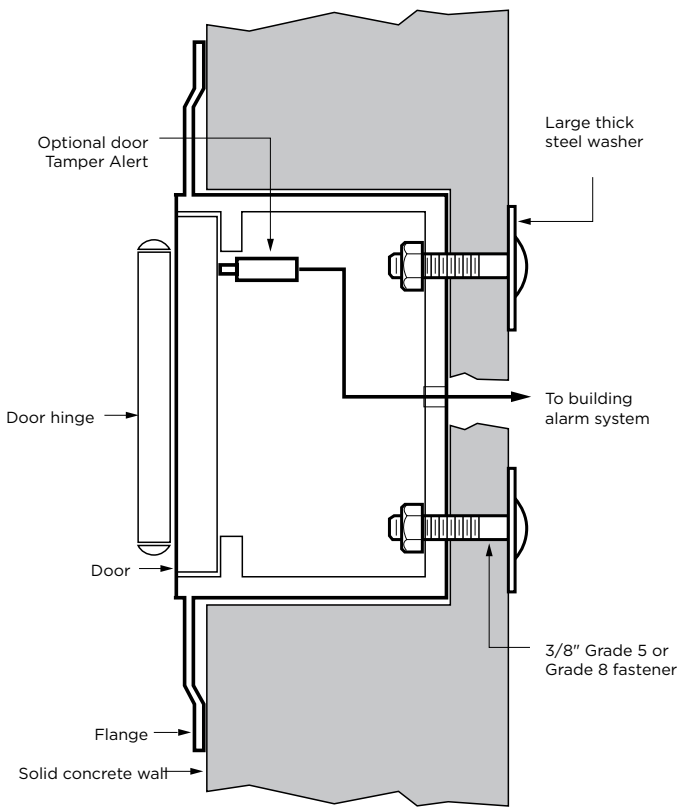
Recess Mounted Models
