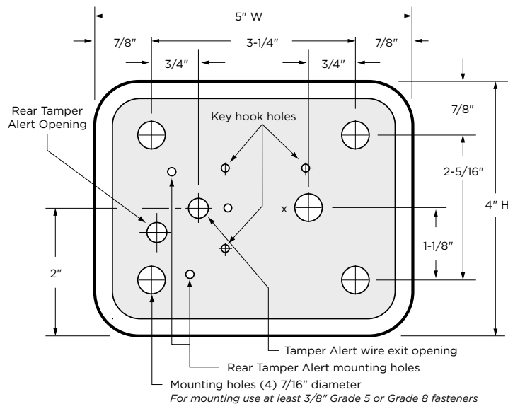
Inside View of Back Plate
